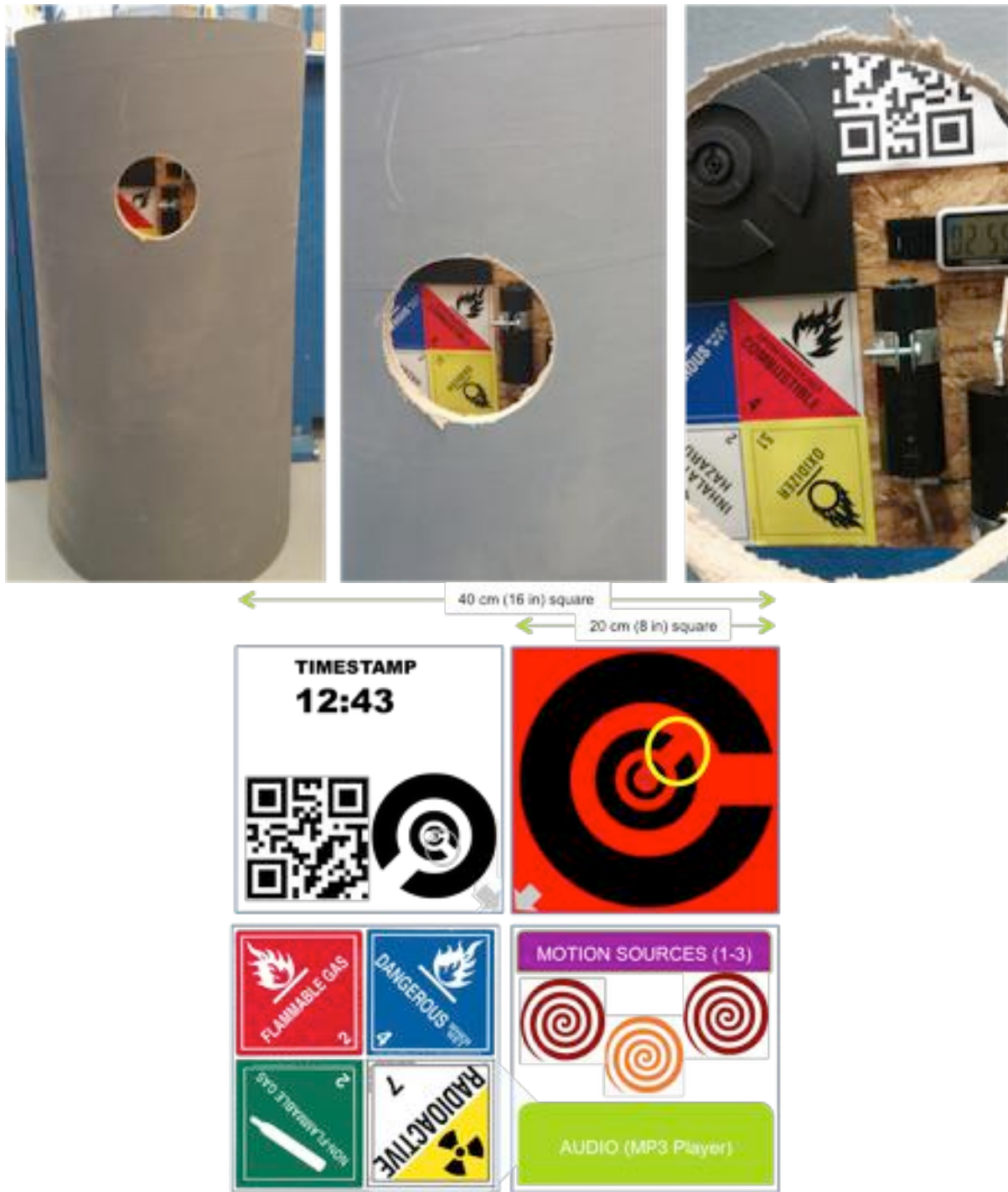
Figure 2: Identification Tasks.
