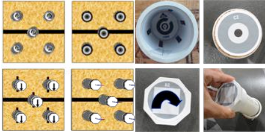
Figure 3: Dexterity tasks
